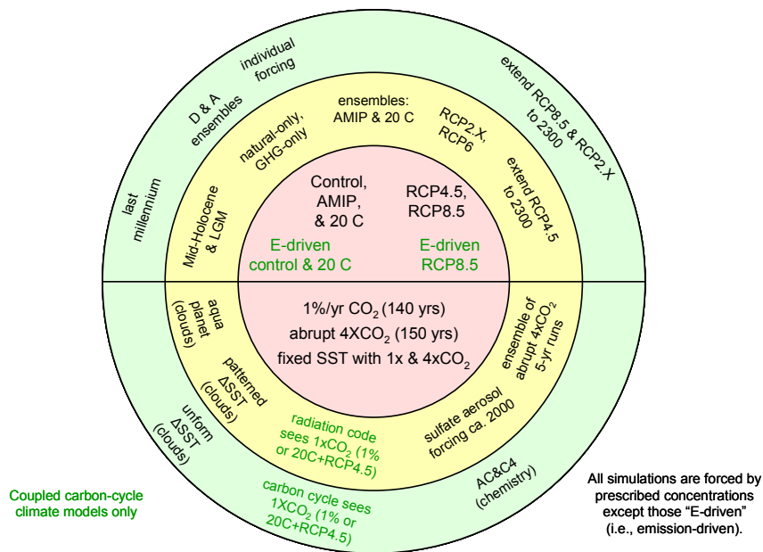
Figure 3: Schematic summary of CMIP5 long-term experiments.
