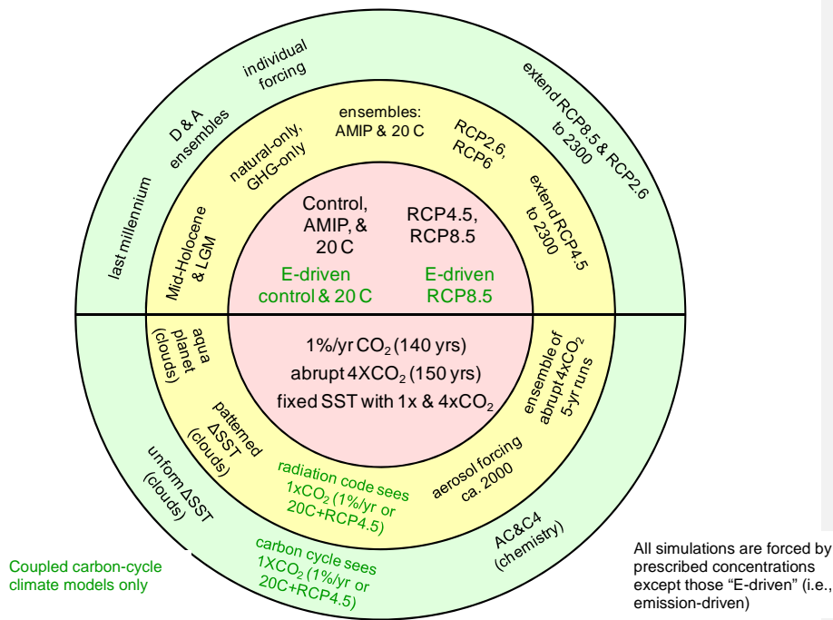
Figure 3: Schematic summary of CMIP5 long-term experiments.
